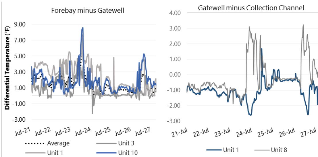
Figure 5 Average Differential Temperatures across Three Dam Locations from July 21–27
