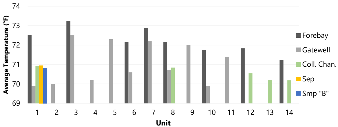
Figure 3 Average Weekly Water Temperatures by Position for five Dam Locations from July 21–27
