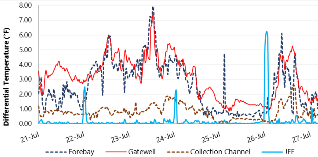
Figure 4 Average Differential Temperatures within four Dam Locations from July 21–27
